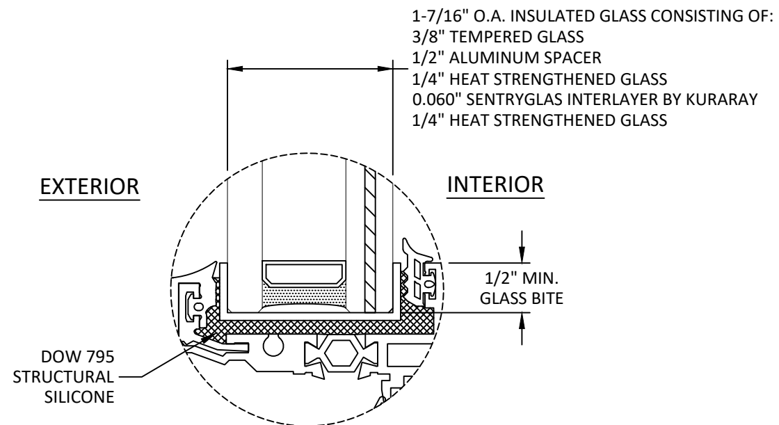
GLAZING DETAIL 1
